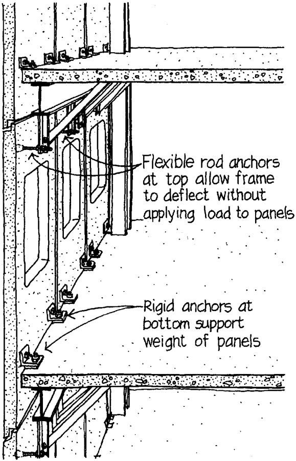
Structure-enclosure joint: Curtain wall panels 18.7
