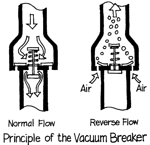
Principle of the Vacuum Breaker
