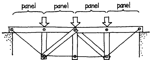
Compression diagonals
