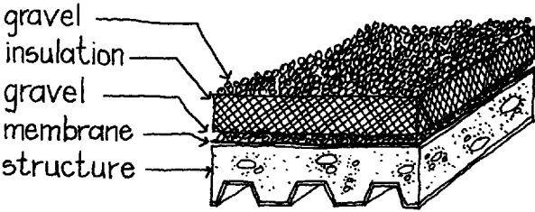
Inverted Roof
