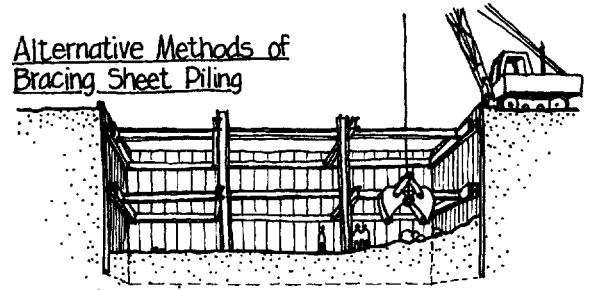
1. Cross-lot bracing
