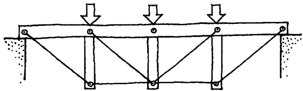
Tension diagonals
